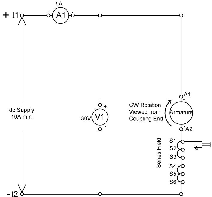
Circuit Diagram Showing connections for demonstrating the variation in RPM for change in series field flux
