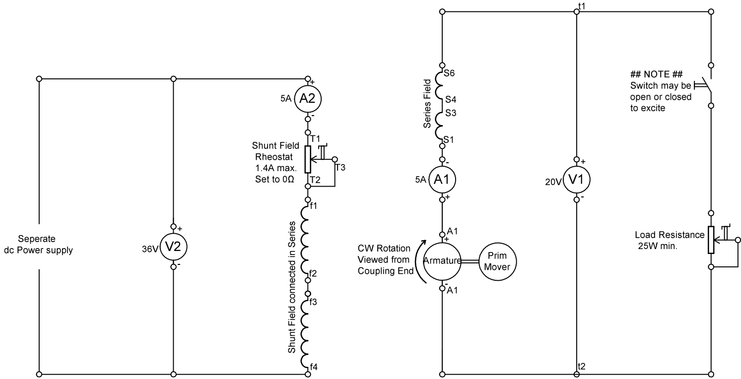
Circuit Diagram Showing conections for demonstrating the Separately excited shunt Generator
