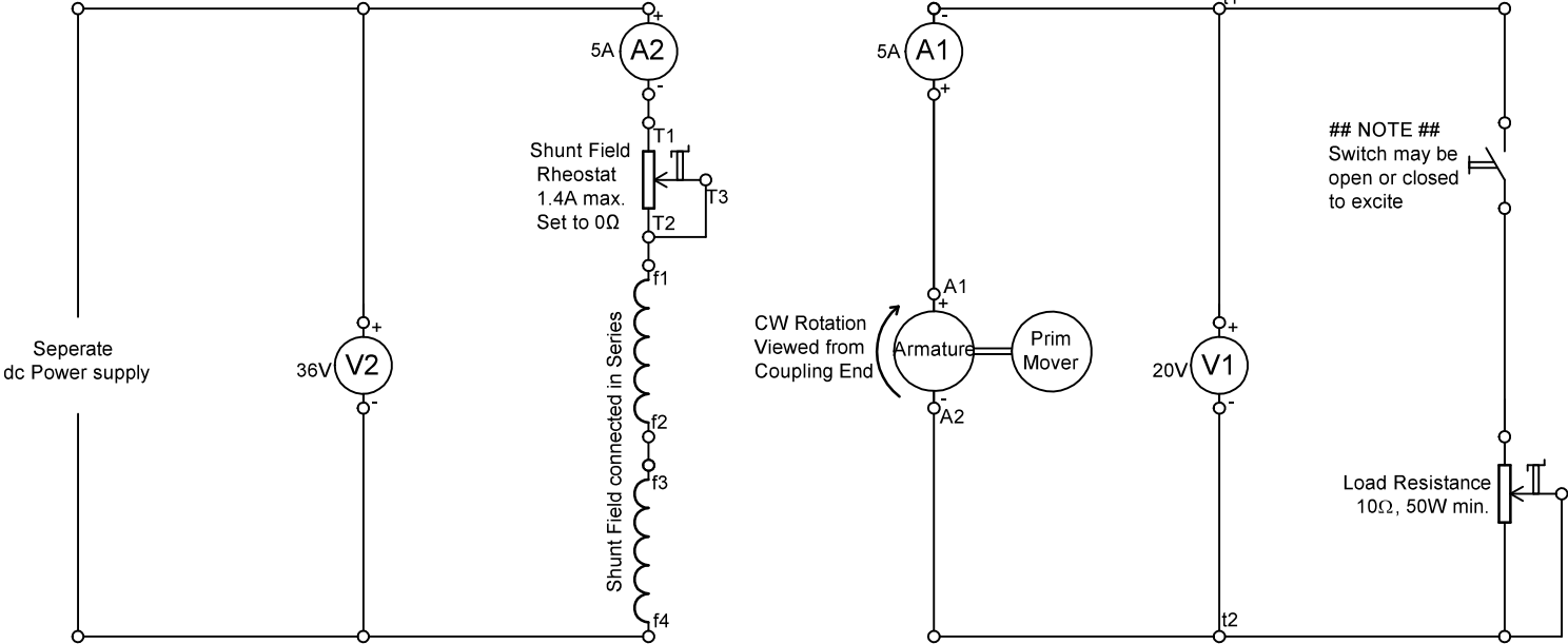
Circuit Diagram Showing conections for demonstrating the Seperately excited shunt Generator
